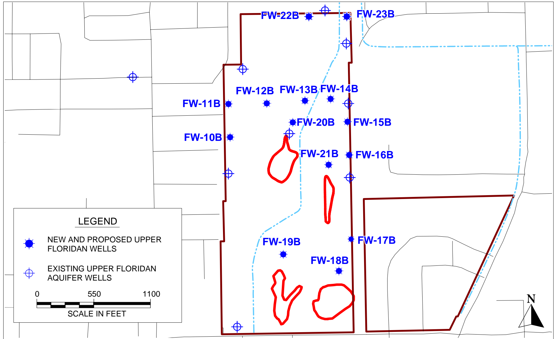
FIGURE 1. LOCATIONS OF EXISTING, NEW, AND PROPOSED UPPER FLORIDAN AQUIFER WELLS
