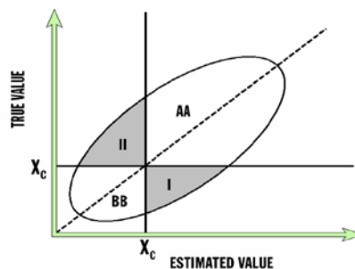
Figure 8. Misclassification Ellipse
